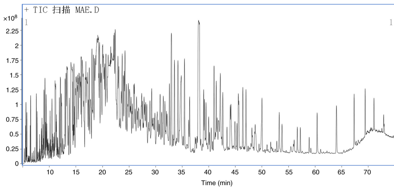
Figure S1. Gas chromatography-mass spectrometry total ion current diagram of pine needle essential oil extracted by microwave-assisted extraction.
