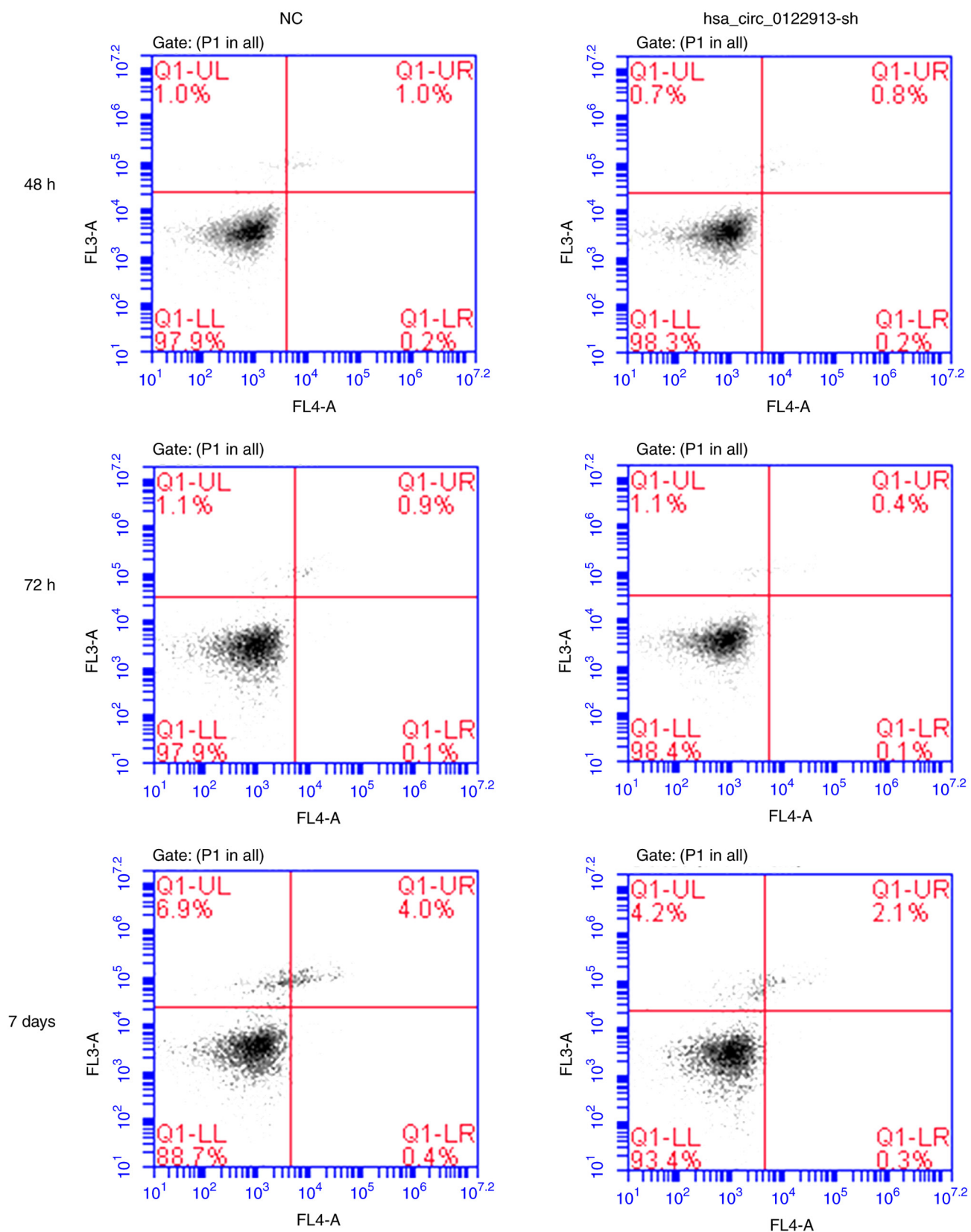
Figure S1. Flow cytometric analysis of apoptosis in the hsa_circ_0122913-knockdown BMSC group at 48, 72 h and 7 days. BMSC, bone marrow mesenchymal stem cell.
