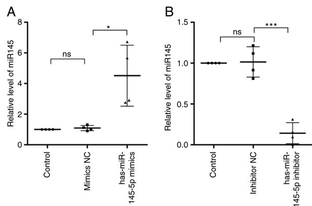
Figure S1. Validation of miR-145 overexpression and knock-down efficiency by reverse transcription-quantitative PCR. (A) Relative expression of miR-145 in cells transfected with miR-145 mimics compared with mimic NC. (B) Relative expression of miR-145 in cells transfected with miR-145 inhibitor compared with inhibitor NC. * P < 0.05 , *** P < 0.001 miR, microRNA; NC, negative control.
