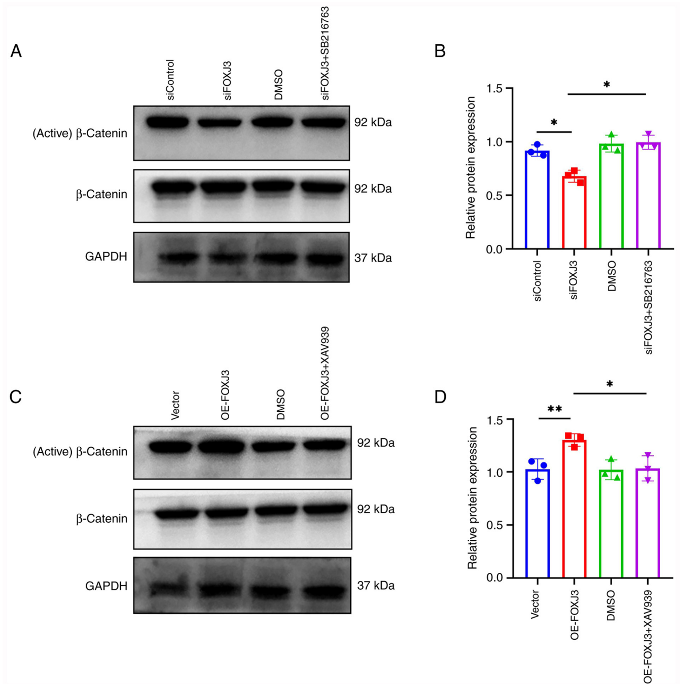
Figure S1. Changes in Wnt/ \beta -catenin pathway expression in rescue experiments. (A) Western blotting detected changes in \beta -catenin expression after FOXJ3 knockdown and treatment with the Wnt/ \beta -catenin pathway agonist SB216763. (B) The protein quantification results for panel A (n=3 biologically independent samples). (C) Western blotting detected changes in \beta -catenin expression after FOXJ3 OE and treatment with the Wnt/ \beta -catenin pathway inhibitor XAV939. (D) The protein quantification results (n=3 biologically independent samples). *P<0.05, **P<0.01. FOXJ3, forkhead box J3; OE, overexpression; si, small interfering.
