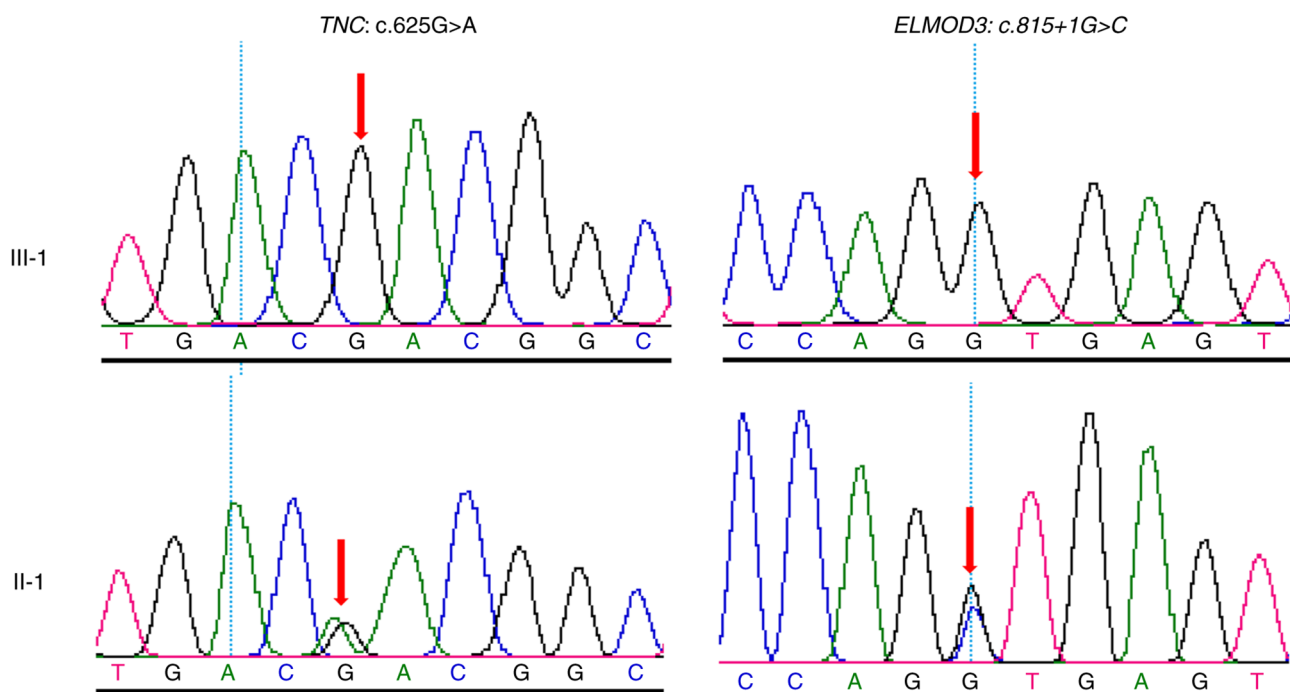
Figure S1. Sanger sequencing. The results of the Sanger sequencing confirm the presence of mutations TNC c.625G>A and ELMOD3 c.815+1G>C in the affected mother (II-1) but not the proband (III-1). The red arrows indicate the mutation site.
