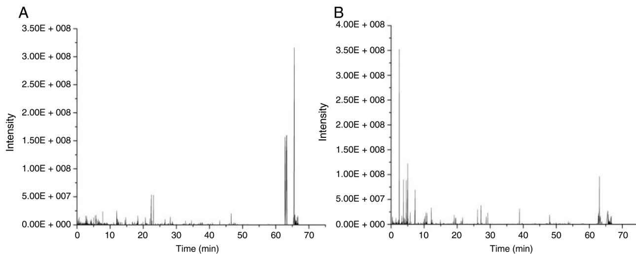
Figure S1. UPLC-Q-TOF/MS BPC-positive ionization pattern of tonic extract samples (A: aqueous extract; B: ethanol extract). UPLC-Q-TOF/MS, ultra-high-performance liquid chromatography-triple/time-of-flight mass spectrometry; BPC, base peak ion current.
