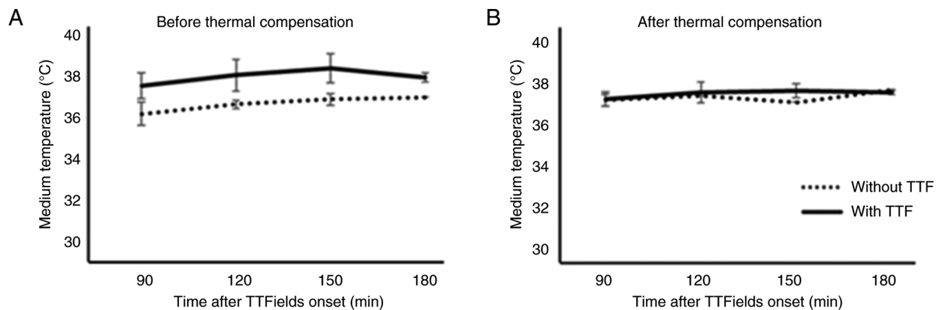
Figure S1. Temperature monitoring during TTFIELDS exposure before and after thermal compensation. (A) Medium temperature profiles measured during TTFIELDS exposure prior to thermal compensation. A modest increase in medium temperature was observed compared with the control condition. (B) Temperature profiles after thermal compensation achieved by incubator adjustment. Similar temperature profiles were maintained between control and TTFIELDS-exposed cultures throughout the exposure period. TTFIELDS, tumor treating fields.
