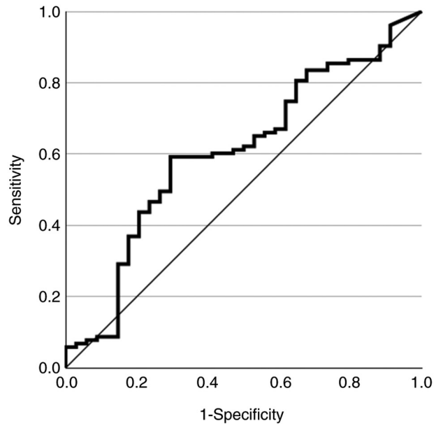
Figure S1. Receiver operating characteristic curve analysis for angiotensin-like 4 expression. The optimal cut-off value (7.7%) was determined by maximizing Youden's index.
