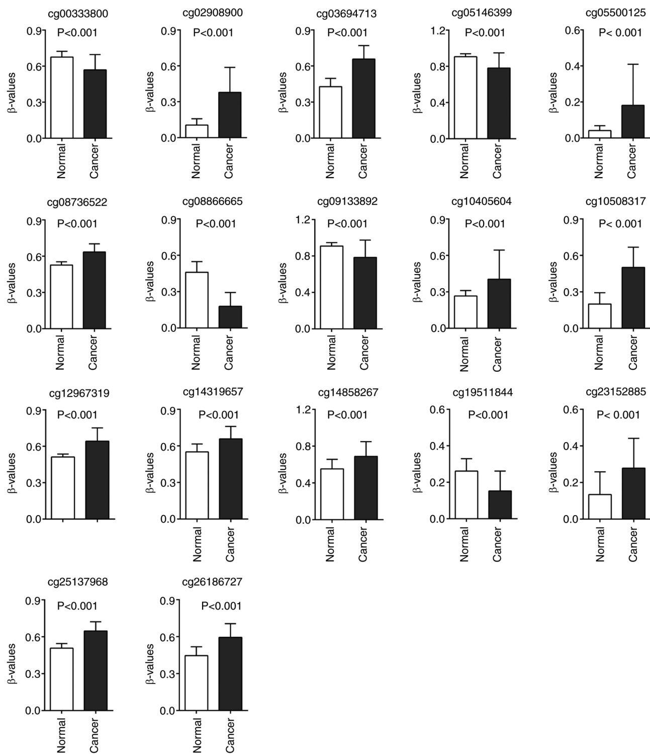
Figure SI. Difference in \beta -values of the 17 CpG sites of the methylation-based classifier between colon adenocarcinoma and normal adjacent tissues.
