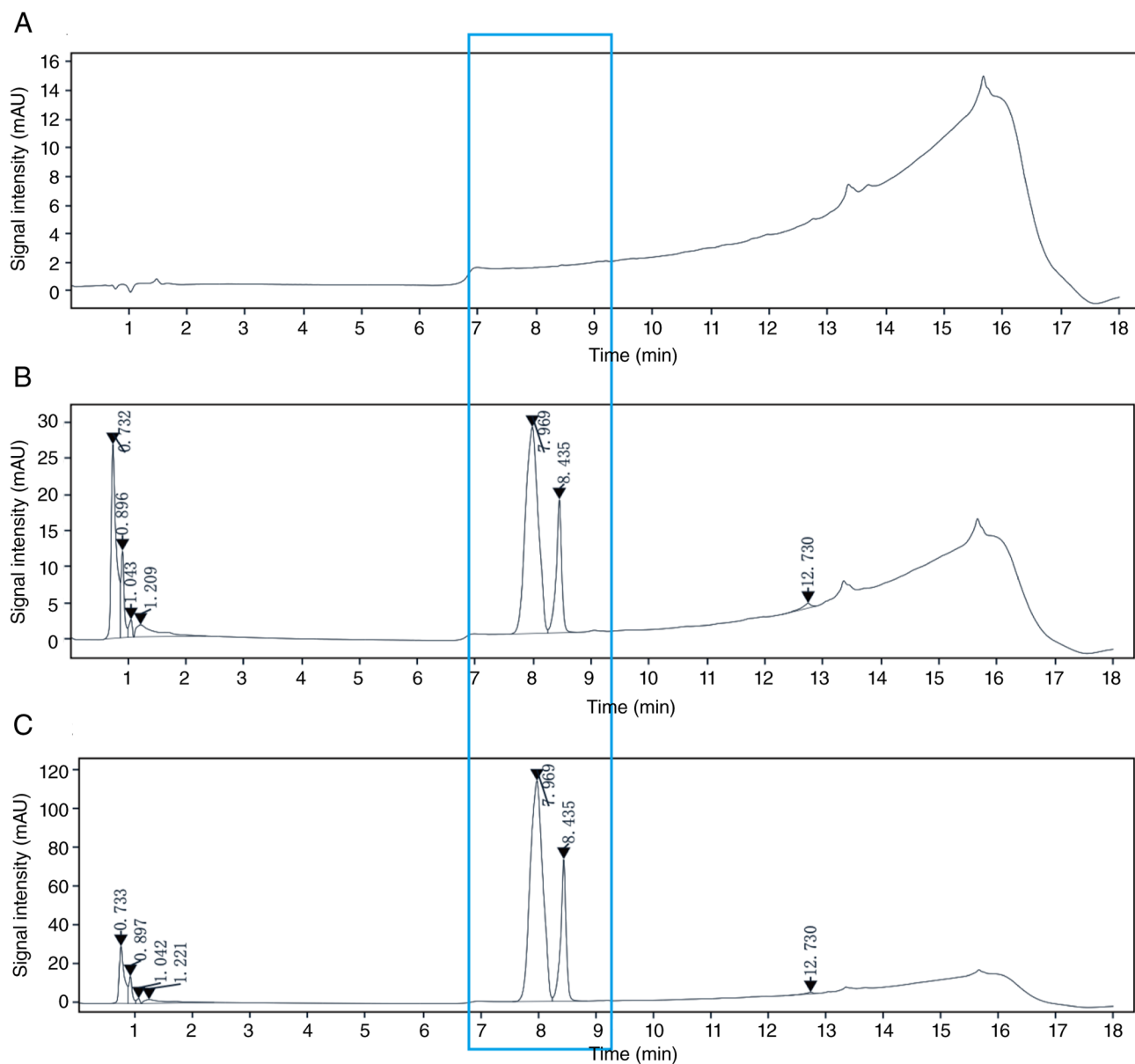
Figure S1. Results of high-performance liquid chromatography showing the detection of Aln. (A) Blank control. (B) Aln. (C) Strontium-based metal organic frameworks loaded with Aln. The blue box indicates the characteristic absorption peaks of Aln. Aln, alendronate sodium.
