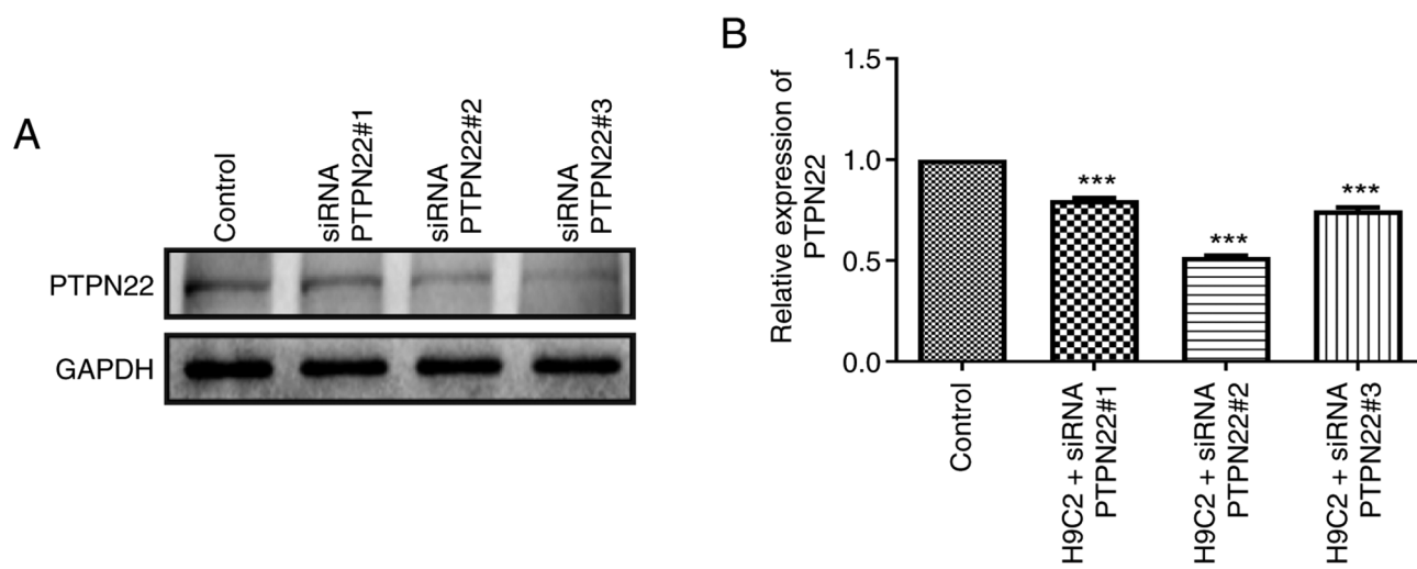
Figure S1. Knockdown efficiency of three siRNAs targeting PTPN22. (A) Western blotting of (B) PTPN22 expression following treatment with siRNA. *** P < 0.0001 vs. control. si, small interfering; PTPN, protein tyrosine phosphatase non-receptor type.
