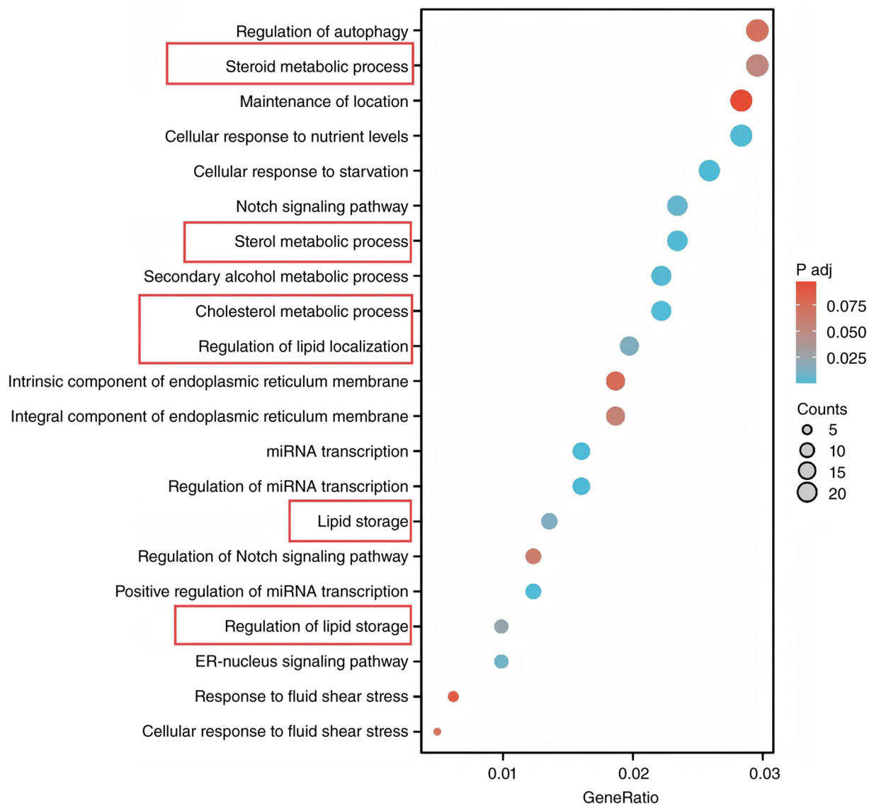
Figure S1. Gene Ontology functional enrichment analysis of differentially expressed proteins identified from DOX-treated AC-16 cell. P adj denotes the adjusted P-value (Bézan-Hochberg correction). Pathways with a red border indicate an association with lipid metabolism enrichment (P adj <0.05). DOX, doxorubicin; P adj, adjusted P-value.
