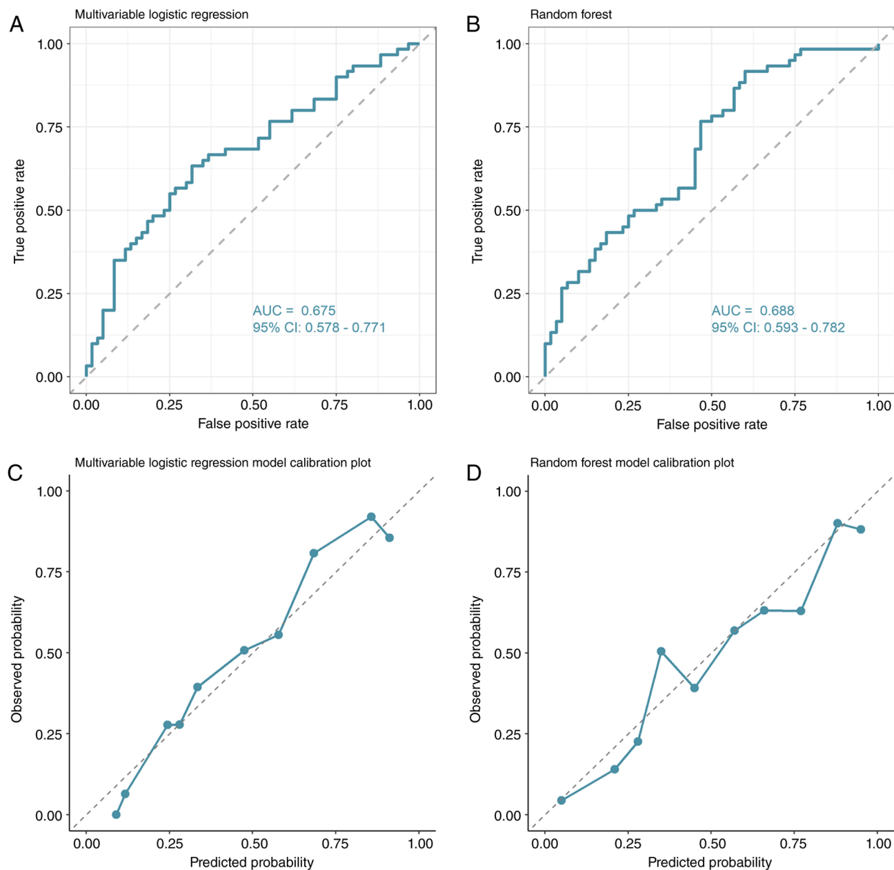
Figure S1. Performance evaluation in the external validation set (A) ROC curve of MLR in the external validation set. (B) ROC curve of RF in the external validation set. (C) Calibration curve of MLR. (D) Calibration curve of RF. MLR, multivariate logistic regression; RF, random forest.
