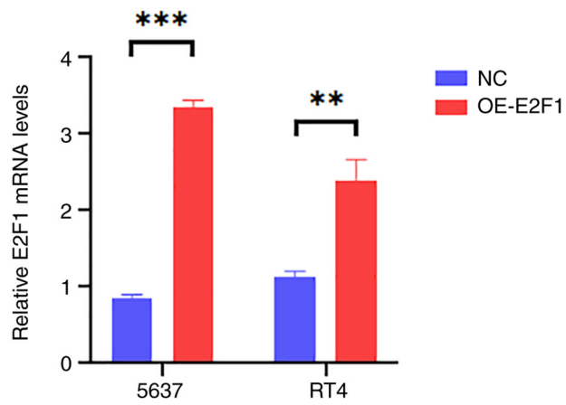
Figure S1. Overexpression efficiency of E2F1 in 5637 cells and RT4 cells. **P<0.01; ***P<0.001. E2F1, E2F transcription factor 1; OE, overexpression; NC, negative control.
